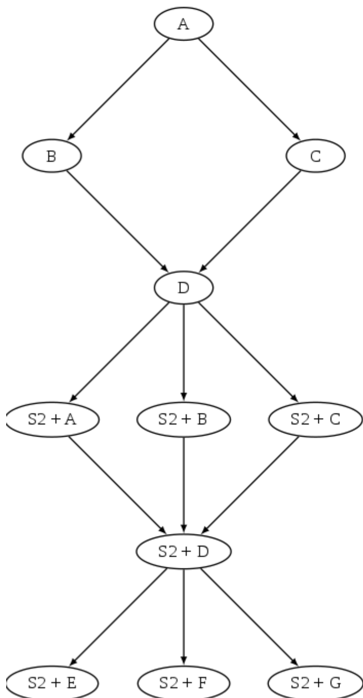
Fig. 6: The complex splice example DAG.
