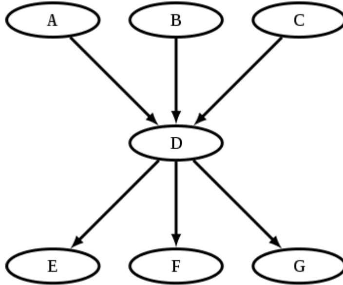
Fig. 4: The X-shaped DAG.
